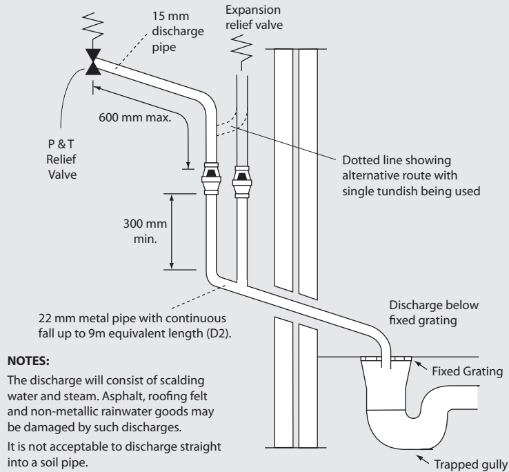
Typical Discharge Pipe Arrangement
