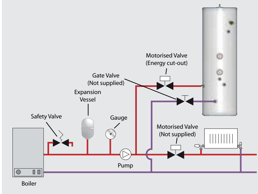
Schematic Sealed Primary System
