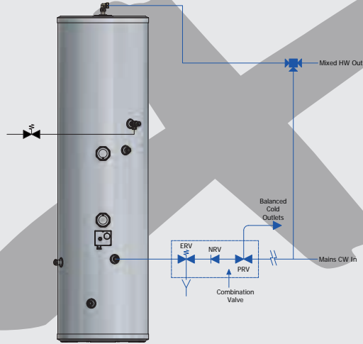
Figure 1: Cold port of the blending valve connected to mains supply NOT ALLOWED
