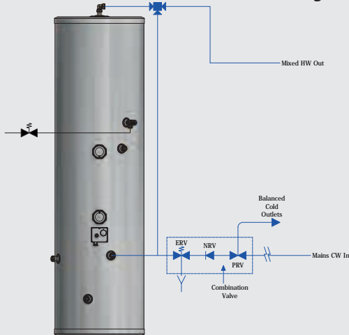
Figure 3: Cold port of the blending valve connected to mains supply to the vessel after the inlet control group
