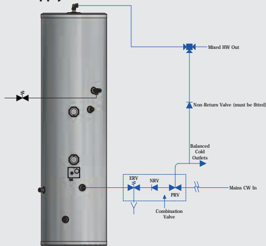
Figure 2: Cold port of the blending valve connected to balanced cold supply - NON-RETURN VALVE MUST BE FITTED
